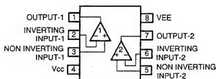
BA15218F NE5532
